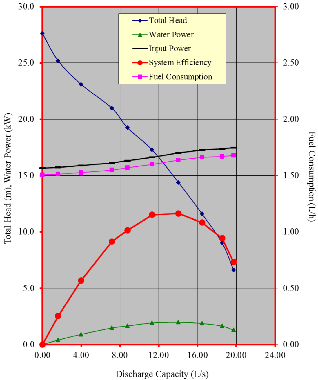
Performance characteristic curves of the KAIAO KDP40 self-priming centrifugal pumpset
